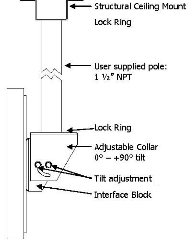
Structural Ceiling Mount
